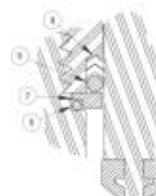
Detail "Y" Enlarged View 1/2" & 3/4" Size Valve
