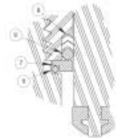
Detail "Y" Enlarged View 1/2" & 3/4" Size Valve
